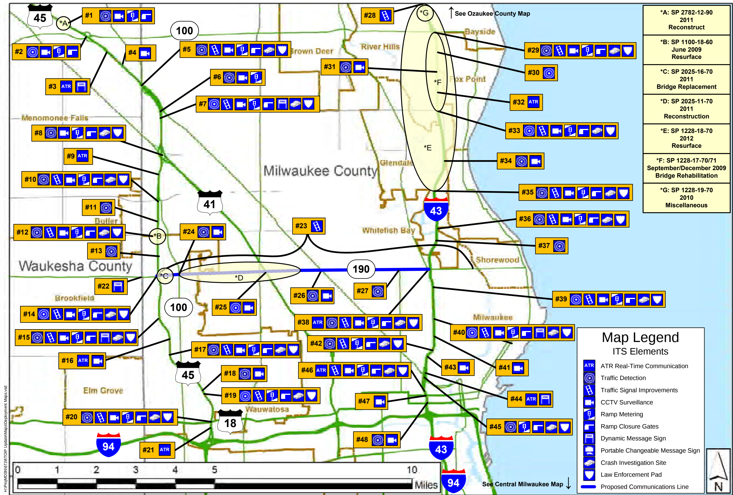
North Milwaukee – TOIP Based ITS Deployment
